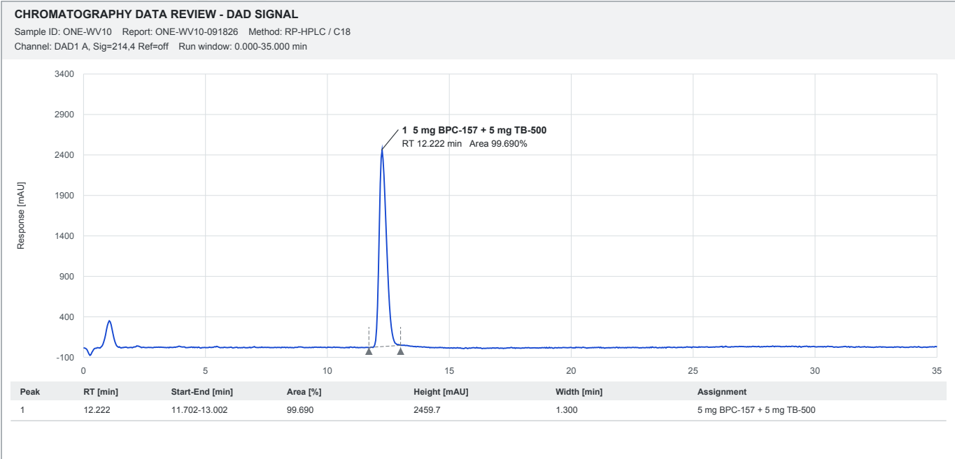
Reconstructed HPLC chromatogram - Wolverine, 5+5 mg
