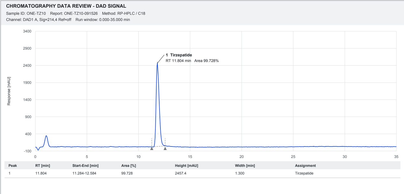
Reconstructed HPLC chromatogram - GLP-2 TZ, 10 mg
