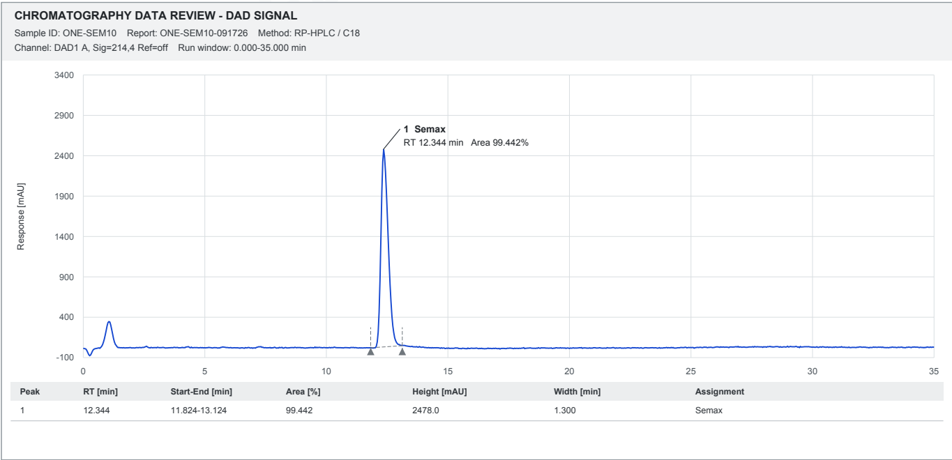
Reconstructed HPLC chromatogram - Semax, 10 mg
