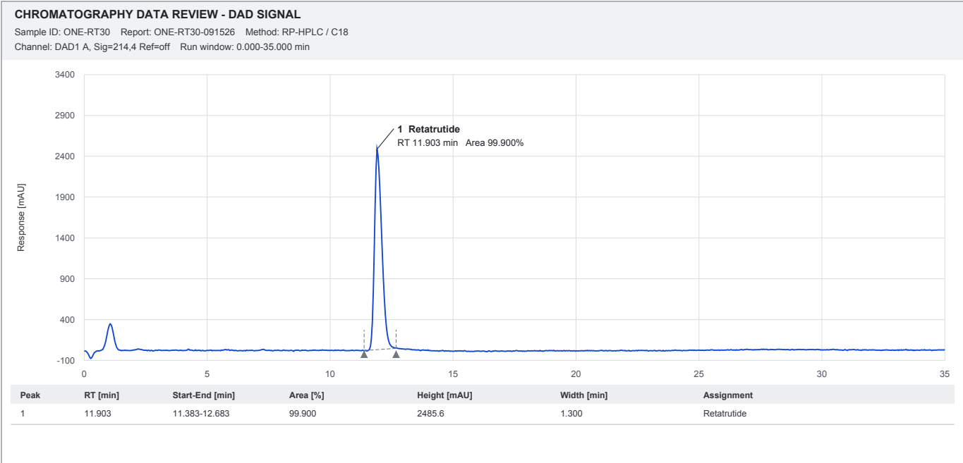
Reconstructed HPLC chromatogram - GLP-3 RT, 30 mg
