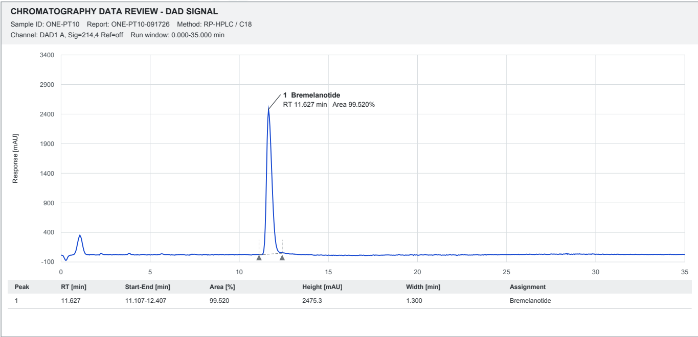
Reconstructed HPLC chromatogram - PT-141, 10 mg
