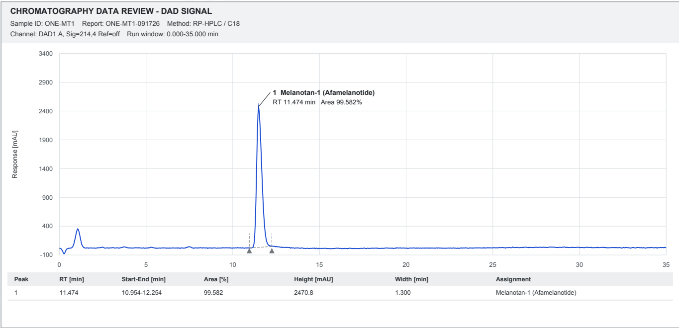
Reconstructed HPLC chromatogram - MT1, 10 mg
