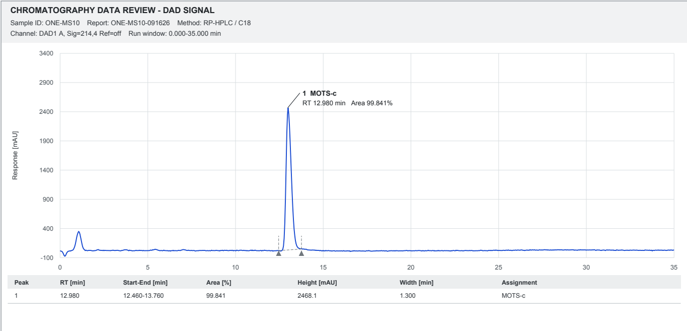
Reconstructed HPLC chromatogram - MOTS-c, 10 mg
