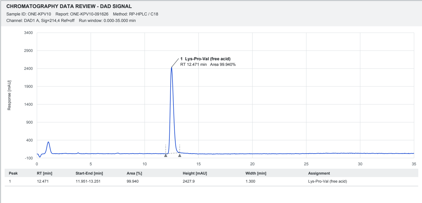
Reconstructed HPLC chromatogram - KPV, 10 mg
