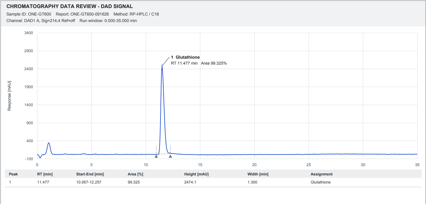
Reconstructed HPLC chromatogram - Glutathione, 600 mg
