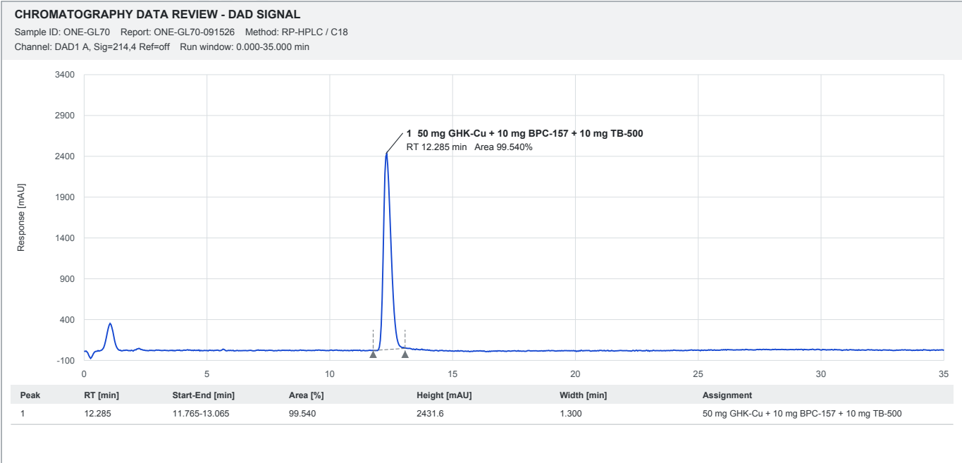
Reconstructed HPLC chromatogram - GLOW, 70 mg
