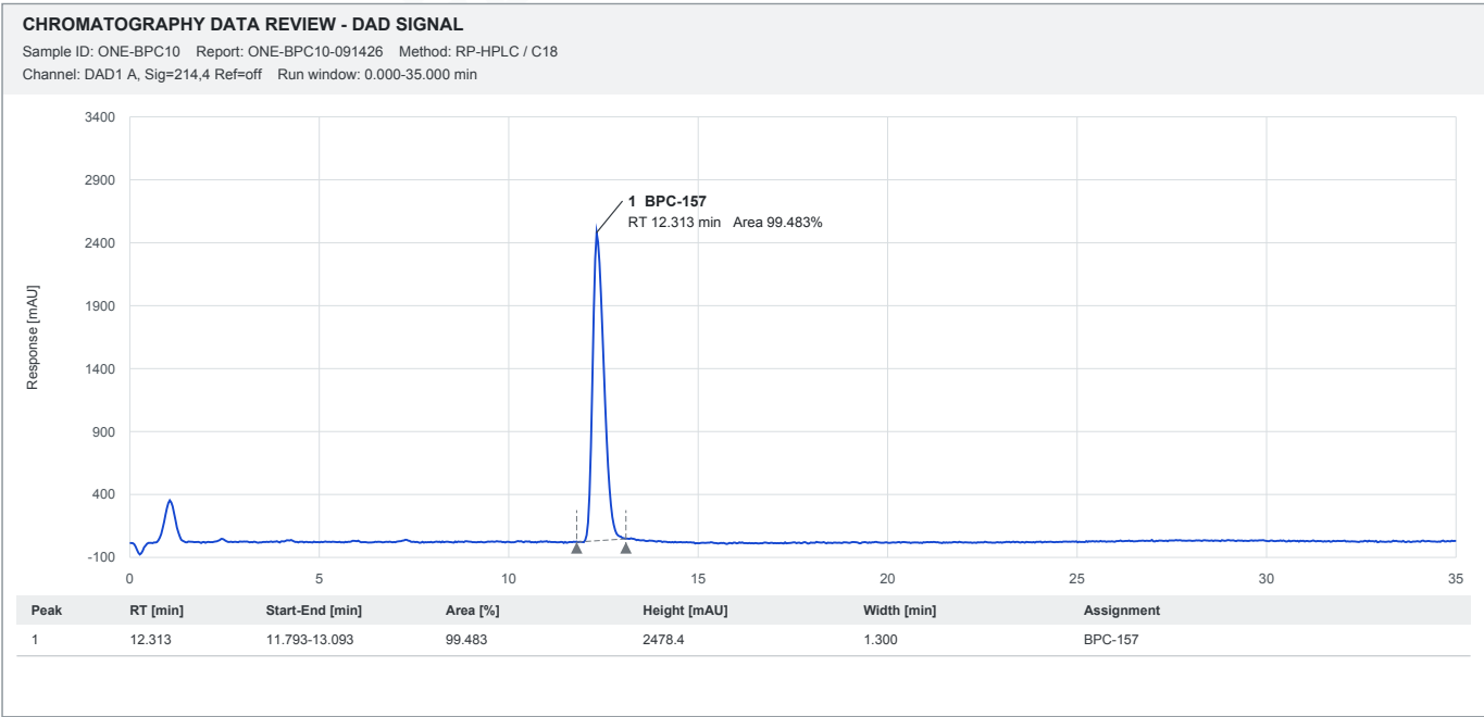
Reconstructed HPLC chromatogram - BPC-157, 10 mg
