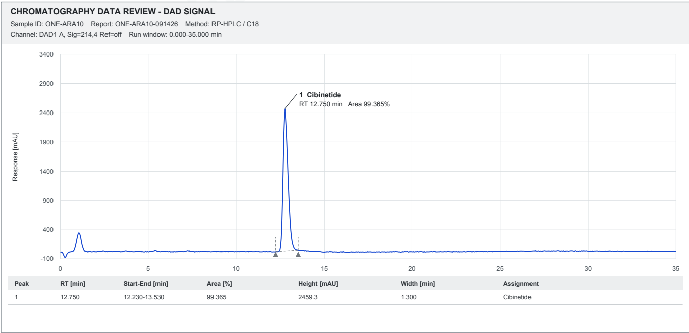
Reconstructed HPLC chromatogram - ARA-290, 10 mg
